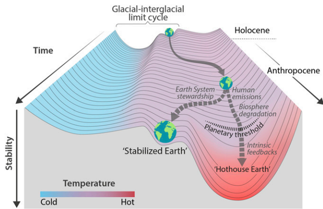
Fig. 2. Stability landscape showing the pathway of the Earth System out of the Holocone and thus, out of the glacial–interglacial limit cycle to its present position in the hotter Anthropocene. The fork in the road in Fig. 1 is shown here as the two divergent pathways of the Earth System in the future (broken arrows). Currently, the Earth System is on a Hothouse Earth pathway driven by human emissions of greenhouse gases and biosphere degradation toward a planetary threshold at \sim 2^\circ\text{C} (horizontal broken line at 2^\circ\text{C} in Fig. 1), beyond which the system follows an essentially irreversible pathway driven by intrinsic biogeophysical feedbacks. The other pathway leads to Stabilized Earth, a pathway of Earth System stewardship guided by human-created feedbacks to a quasistable, human-maintained basin of attraction. “Stability” (vertical axis) is defined here as the inverse of the potential energy of the system. Systems in a highly stable state (deep valley) have low potential energy, and considerable energy is required to move them out of this stable state. Systems in an unstable state (top of a hill) have high potential energy, and they require only a little additional energy to push them off the hill and down toward a valley of lower potential energy.
